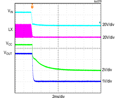
MAXM17632 SHUTDOWN THROUGH V_{IN} V_{OUT} = 2.5V , f_{SW} = 700kHz , FULL LOAD, PWM MODE
