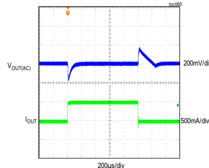
MAXM17631/MAXM17632 LOAD-TRANSIENT RESPONSE V_{OUT} = 5V , f_{SW} = 1250kHz , DCM MODE (LOAD CURRENT STEPPED FROM 10mA TO 0.5A)
