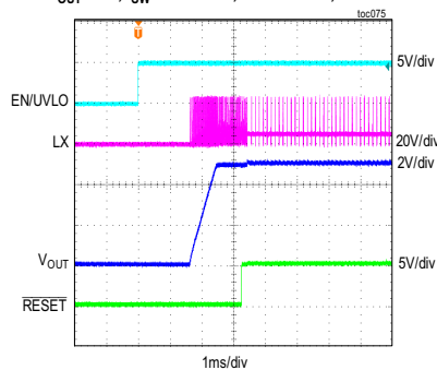
MAXM17631/MAXM17632 STARTUP THROUGH ENABLE V_{OUT} = 5V , f_{SW} = 1250kHz , 10mA LOAD, PFM MODE
