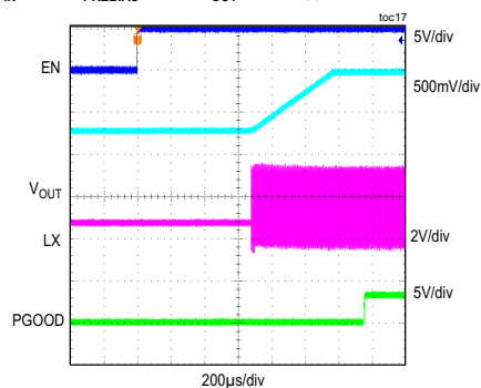
MAXM17623 STARTUP INTO PRE-BIAS V_{IN} = 3.3V , V_{PREBIAS} = 0.8V , V_{OUT} = 1.5V , I_{OUT} = 1A , \text{PWM MODE}
