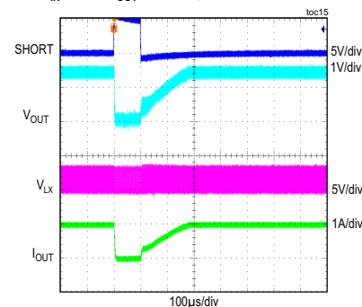
MAXM17623 TEMPORARY OUTPUT SHORT V_{IN} = 3.3V , V_{OUT} = 1.5V , I_{LOAD} = 1A , \text{MODE} = \text{PWM}
