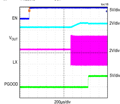
MAXM17624 STARTUP INTO PRE-BIAS V_{IN} = 5V , V_{PREBIAS} = 2.5V , V_{OUT} = 3.3V , I_{LOAD} = 1A , \text{PWM MODE}
