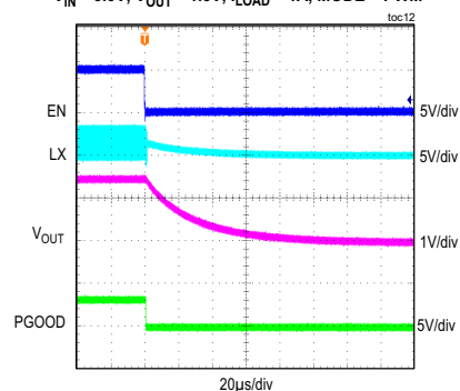
MAXM17623 SHUTDOWN THROUGH ENABLE V_{IN} = 3.3V , V_{OUT} = 1.5V , I_{LOAD} = 1A , \text{MODE} = \text{PWM}
