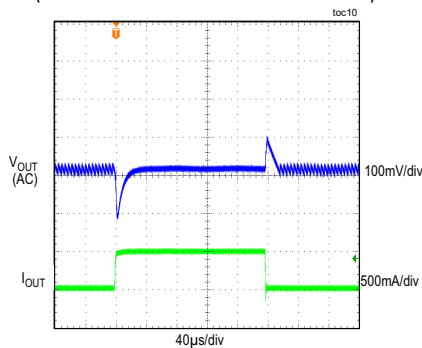
MAXM17624 LOAD TRANSIENT RESPONSE V_{IN} = 5V , V_{OUT} = 3.3V , \text{MODE} = \text{PFM} (LOAD CURRENT STEPPED FROM 0A TO 500mA)
