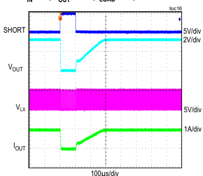
MAXM17624 TEMPORARY OUTPUT SHORT V_{IN} = 5V , V_{OUT} = 3.3V , I_{LOAD} = 1A , \text{MODE} = \text{PWM}
