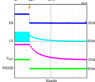
MAXM17624 SHUTDOWN THROUGH ENABLE V_{IN} = 5V , V_{OUT} = 3.3V , I_{LOAD} = 1A , \text{MODE} = \text{PWM}
