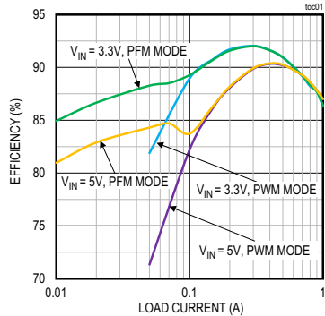
MAXM17623 EFFICIENCY vs. LOAD CURRENT V_{OUT} = 1.5V , PWM & PFM MODE
