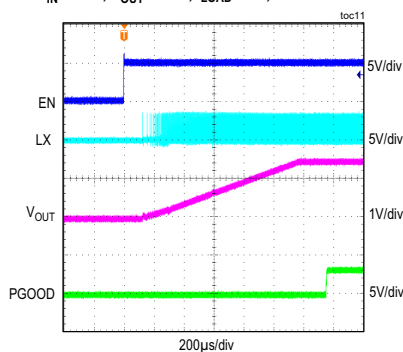
MAXM17623 STARTUP THROUGH ENABLE V_{IN} = 3.3V , V_{OUT} = 1.5V , I_{LOAD} = 1A , \text{MODE} = \text{PWM}
