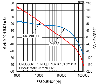
MAXM17623 BODE PLOT V_{IN} = 3.3V , V_{OUT} = 1.5V , FULL LOAD, PWM MODE
