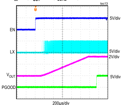
MAXM17624 STARTUP THROUGH ENABLE V_{IN} = 5V , V_{OUT} = 3.3V , I_{LOAD} = 1A , \text{MODE} = \text{PWM}
