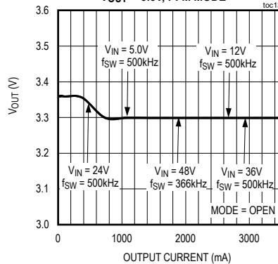
LOAD REGULATION V OUT = 3.3V, PFM MODE
