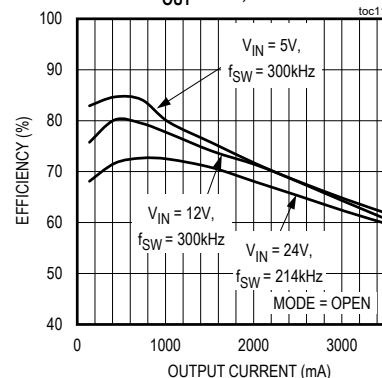
EFFICIENCY vs. OUTPUT CURRENT V OUT = 0.9V, PFM MODE
