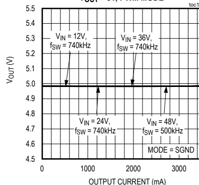
LOAD REGULATION V OUT = 5V, PWM MODE
