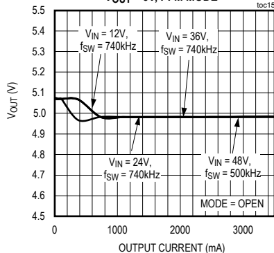
LOAD REGULATION V OUT = 5V, PFM MODE
