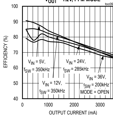
EFFICIENCY vs. OUTPUT CURRENT V OUT = 1.2V, PFM MODE
