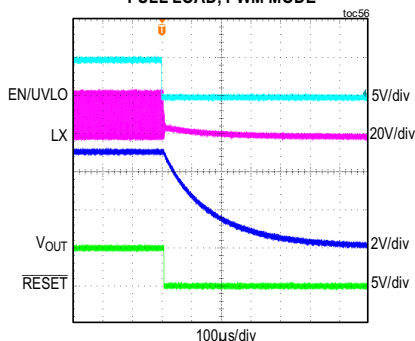
MAXM15462 SHUTDOWN THROUGH ENABLE V_{IN} = 24V , ADJUSTABLE V_{OUT} = 5V , FULL LOAD, PWM MODE
