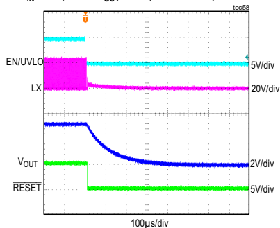
MAXM15463 SHUTDOWN THROUGH ENABLE V_{IN} = 24V , FIXED V_{OUT} = 3.3V , FULL LOAD, PWM MODE
