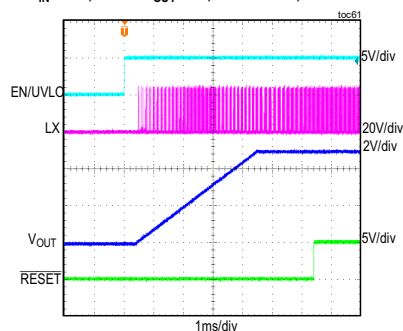
MAXM15464 STARTUP THROUGH ENABLE V_{IN} = 24V , FIXED V_{OUT} = 5V , FULL LOAD, PWM MODE
