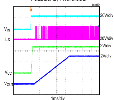
MAXM15462 STARTUP THROUGH V_{IN} V_{IN} = 24V , ADJUSTABLE V_{OUT} = 5V , FULL LOAD, PWM MODE
