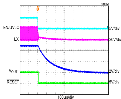
MAXM15464 SHUTDOWN THROUGH ENABLE V_{IN} = 24V , FIXED V_{OUT} = 5V , FULL LOAD, PWM MODE
