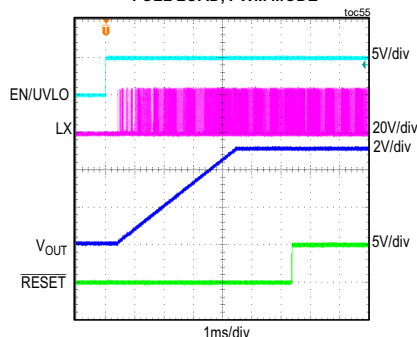
MAXM15462 STARTUP THROUGH ENABLE V_{IN} = 24V , ADJUSTABLE V_{OUT} = 5V , FULL LOAD, PWM MODE
