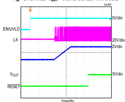
MAXM15464 STARTUP THROUGH ENABLE (2.5V PREBIAS) V_{IN} = 24V , FIXED V_{OUT} = 5V , NO LOAD, PWM MODE
