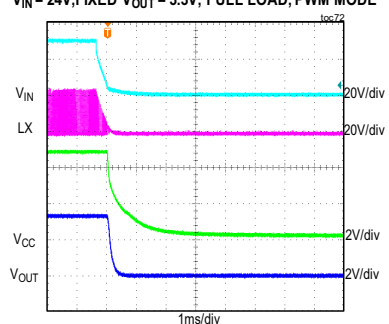
MAXM15463 SHUTDOWN THROUGH V_{IN} V_{IN} = 24V , FIXED V_{OUT} = 3.3V , FULL LOAD, PWM MODE
