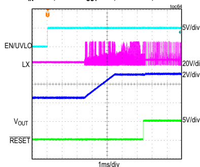
MAXM15464 STARTUP THROUGH ENABLE (2.5V PREBIAS) V_{IN} = 24V , FIXED V_{OUT} = 5V , NO LOAD, PFM MODE
