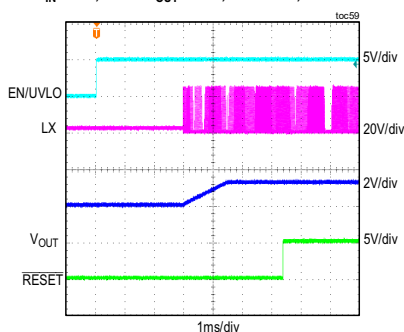
MAXM15463 STARTUP THROUGH ENABLE (2V PREBIAS) V_{IN} = 24V , FIXED V_{OUT} = 3.3V , NO LOAD, PWM MODE
