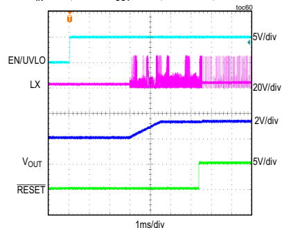
MAXM15463 STARTUP THROUGH ENABLE (2V PREBIAS) V_{IN} = 24V , FIXED V_{OUT} = 3.3V , NO LOAD, PFM MODE
