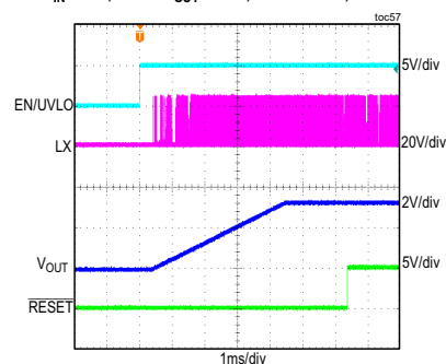
MAXM15463 STARTUP THROUGH ENABLE V_{IN} = 24V , FIXED V_{OUT} = 3.3V , FULL LOAD, PWM MODE
