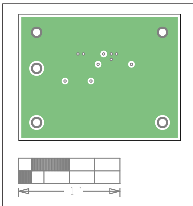
MAXM38643A EV System PCB Layout—Internal2
