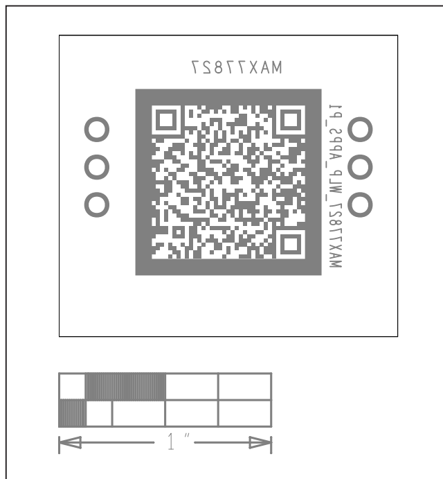
MAX77827A EV System PCB Layout—Bottom Silkscreen
