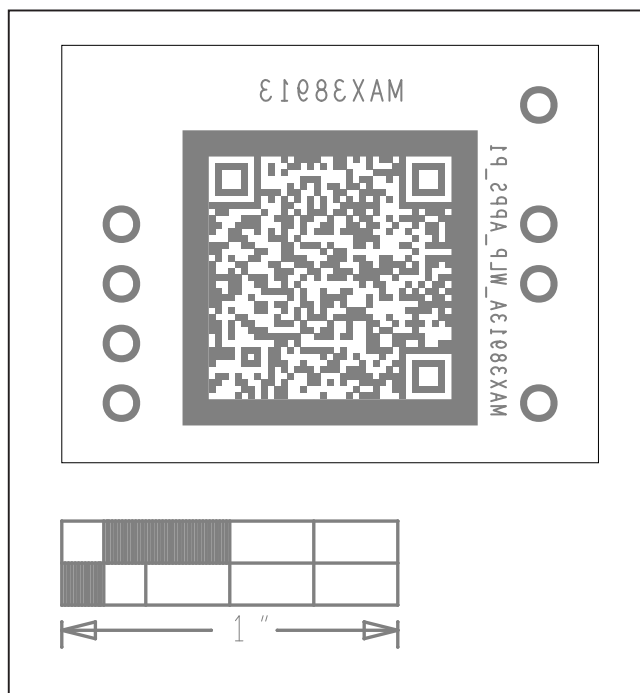
MAX38913 EV System PCB Layout—Bottom Silkscreen
