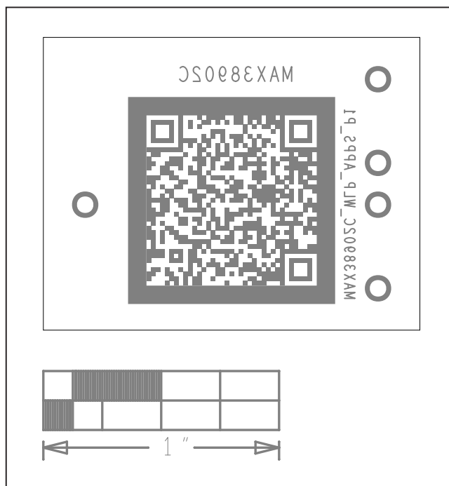
MAX38902C EV System PCB Layout—Bottom Silkscreen
