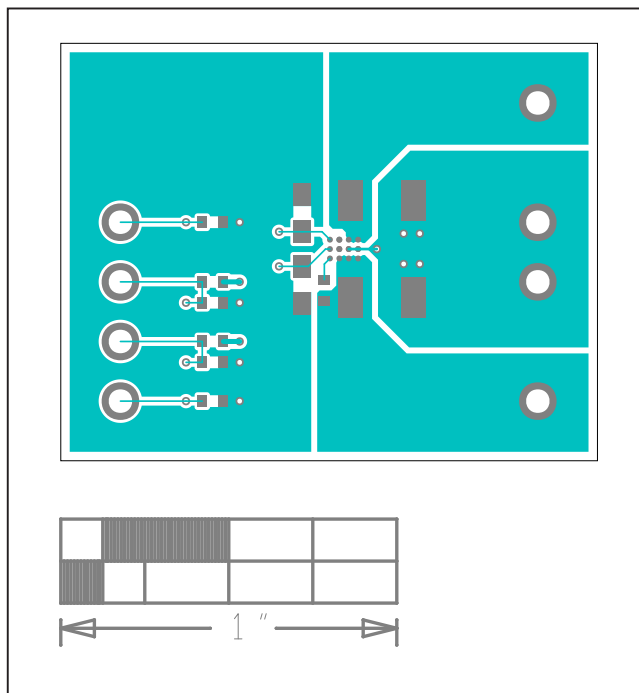
MAX38913 EV System PCB Layout—Top
