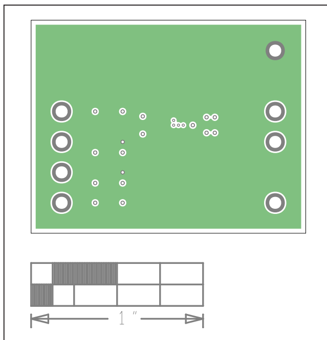
MAX38913 EV System PCB Layout—Internal2
