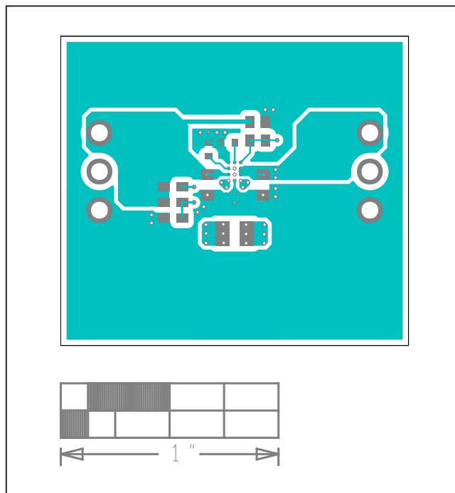
MAX77827A EV System PCB Layout—Top
