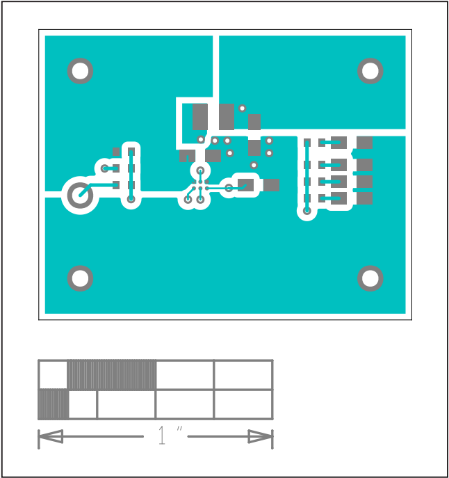
MAX38640A EV System PCB Layout—Top
