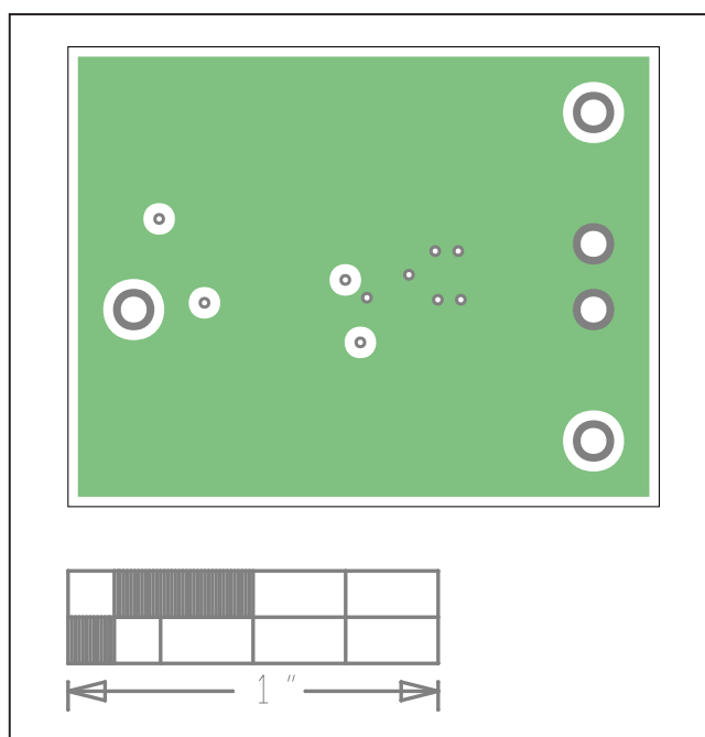
MAX38902C EV System PCB Layout—Internal2
