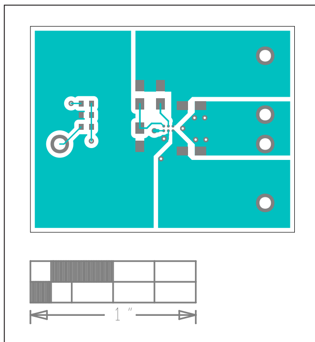
MAX38902C EV System PCB Layout—Top
