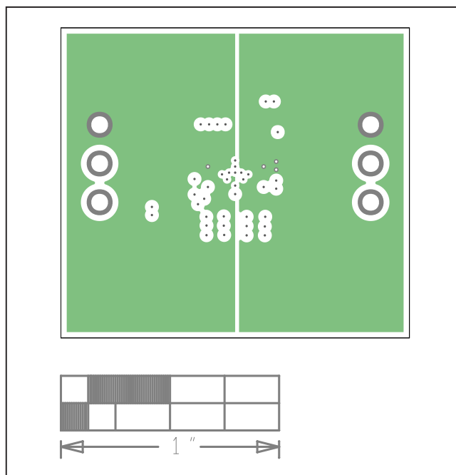
MAX77827A EV System PCB Layout—Internal3
