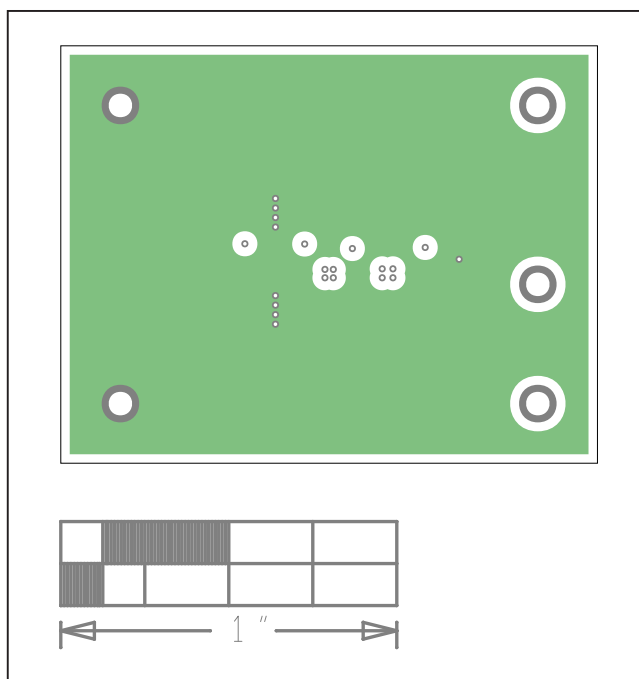
MAX17227A EV System PCB Layout—Internal2
