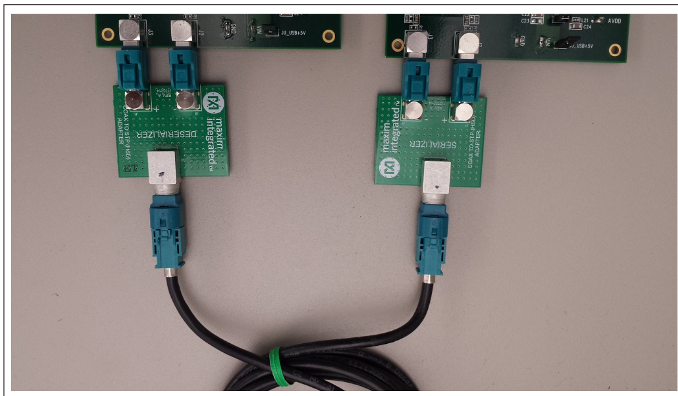
Figure 2. Photo of MAXCOAX2STP-HSD Adapter Kit Setup
