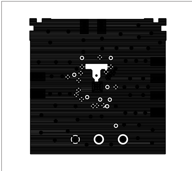
Figure 6. MAX9994 EV Kit PC Board Layout—Inner Layer 2 (GND)
