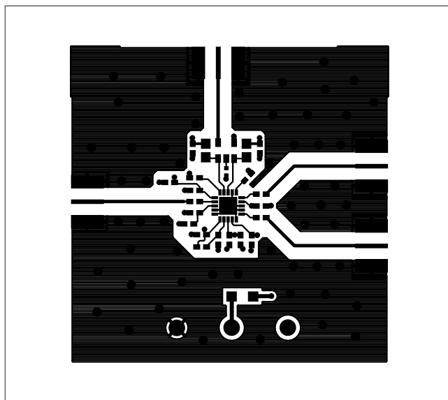
Figure 5. MAX9994 EV Kit PC Board Layout—Top Layer Metal
