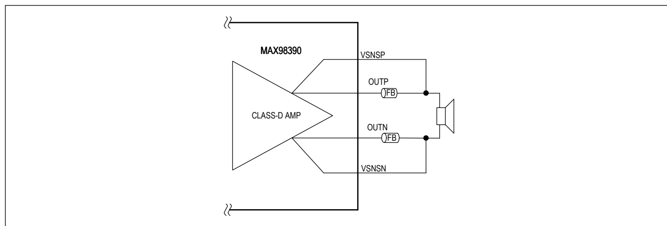
Figure 19. Output Sensing When Using Ferrite Beads
