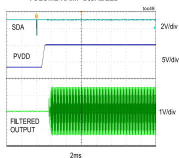
SYSTEM TURN-ON RESPONSE VOLUME RAMP DISABLED
