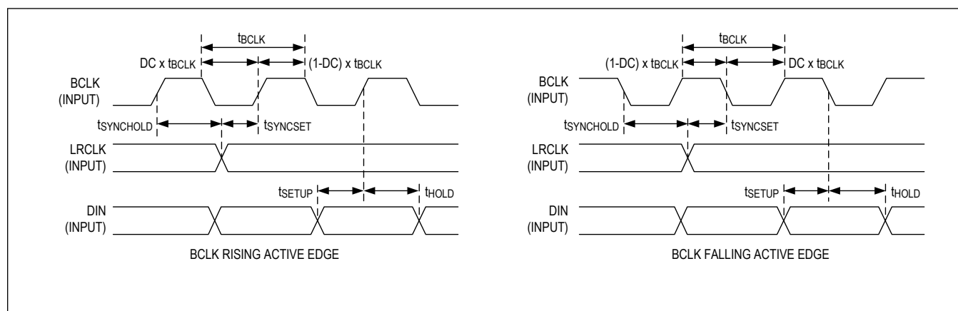
Figure 16. PCM Interface Timing/Slave Mode—LRCLK, BCLK, DIN Timing Diagram
