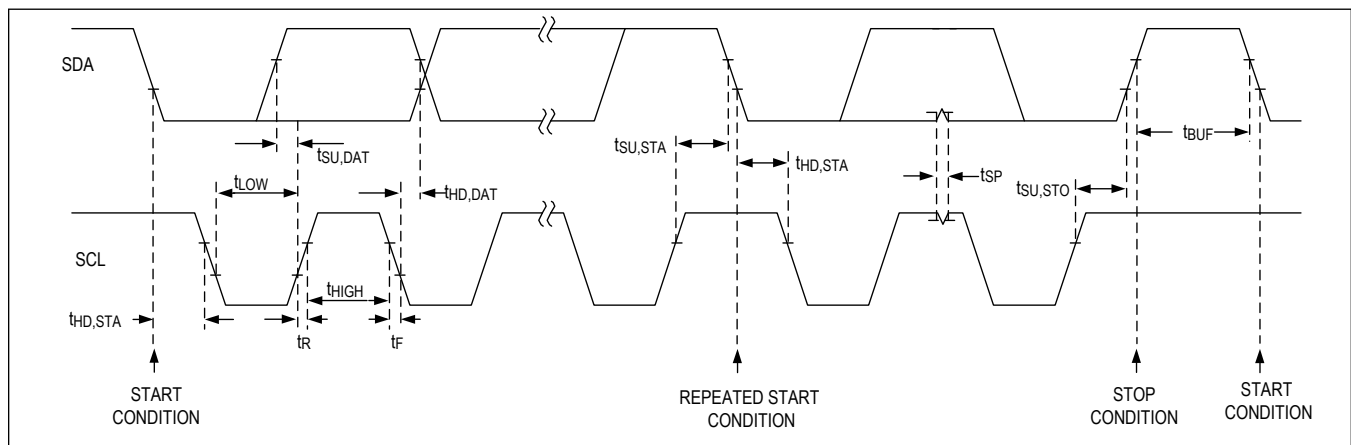
Figure 34. I^2C START, STOP, and REPEATED START Conditions
