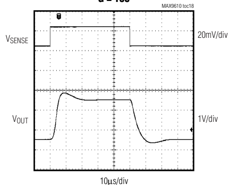
LARGE-SIGNAL RESPONSE
