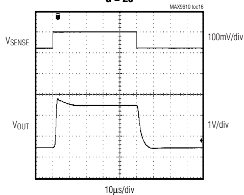
LARGE-SIGNAL RESPONSE
