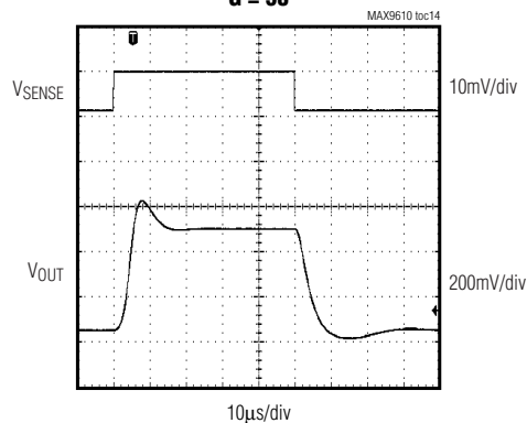
SMALL-SIGNAL RESPONSE
