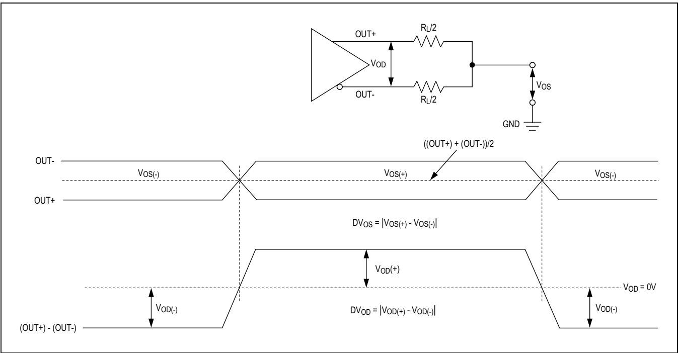
Figure 1. Serial-Output Parameters
