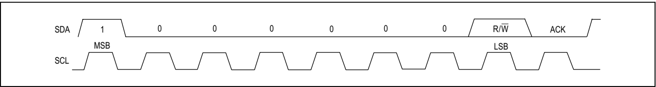
Figure 32. Slave Address
