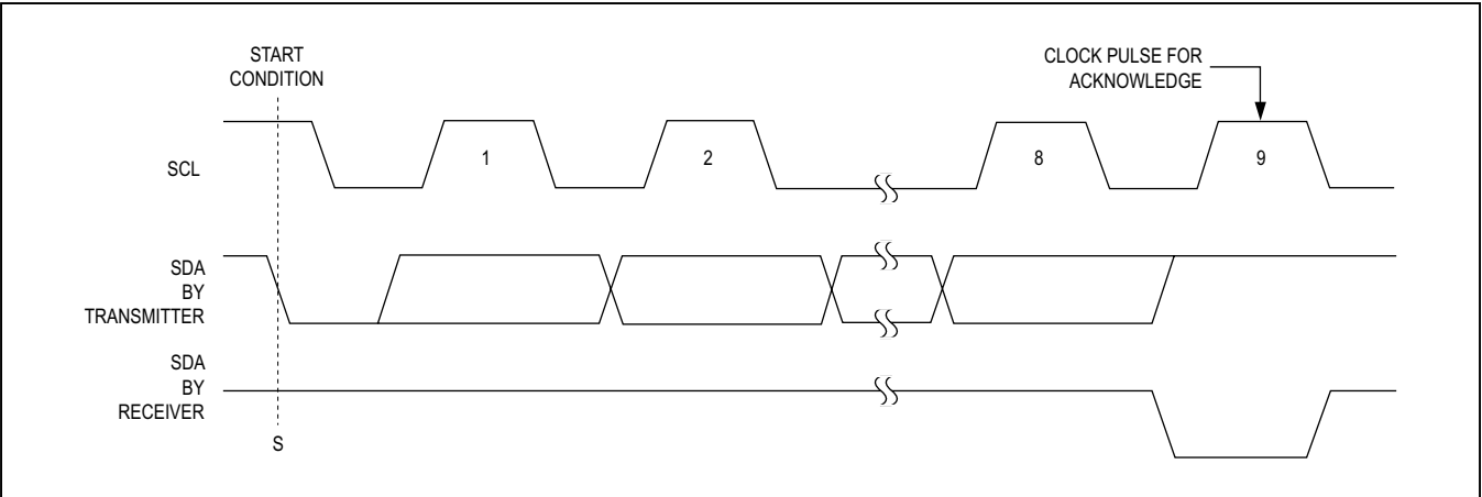
Figure 31. Acknowledge
