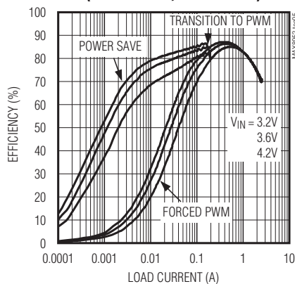
EFFICIENCY vs. LOAD CURRENT (1.1V OUTPUT, 26MHz SYNC)
