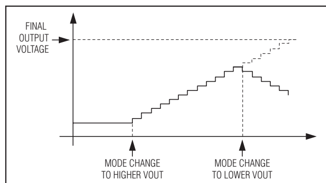
Figure 8. Mode Change Before Final Value is Reached
