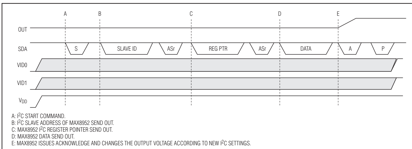
Figure 13. Update Output Operation
