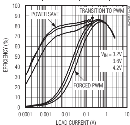
EFFICIENCY vs. LOAD CURRENT (1.0V OUTPUT, 26MHz SYNC)
