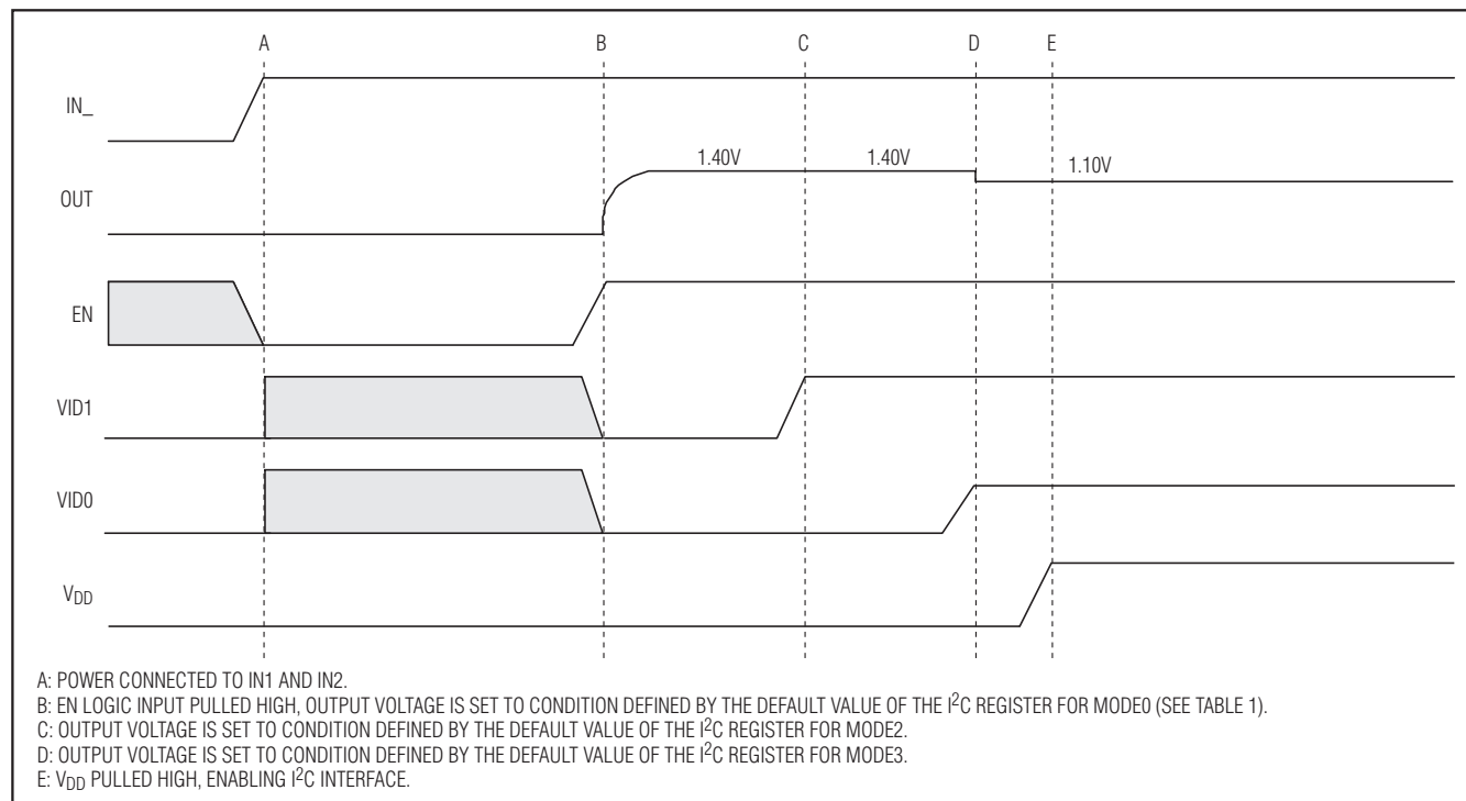
Figure 2. Power-Up Sequence
