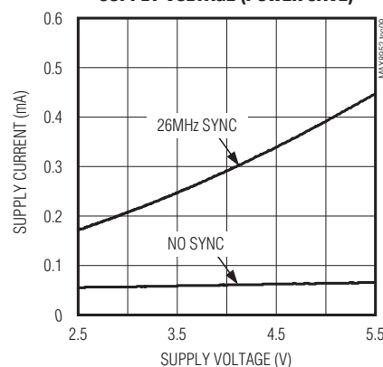
NO-LOAD SUPPLY CURRENT vs. SUPPLY VOLTAGE (POWER SAVE)
