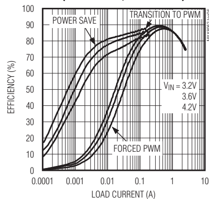
EFFICIENCY vs. LOAD CURRENT (1.4V OUTPUT, 26MHz SYNC)
