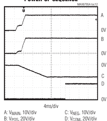
POWER-UP SEQUENCE
