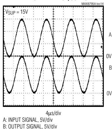
OPERATIONAL-AMPLIFIER RAIL-TO-RAIL INPUT/OUTPUT
