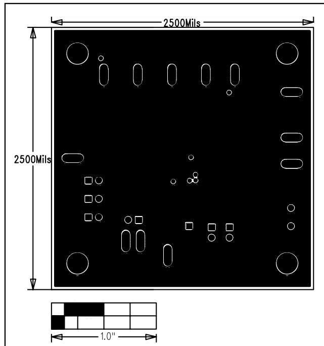
Figure 7. MAX8677A EV Kit PCB Layout—Solder Side
