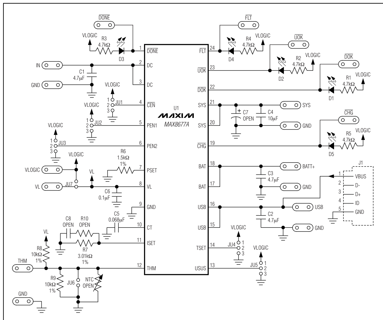
Figure 2. MAX8677A EV Kit Schematic
