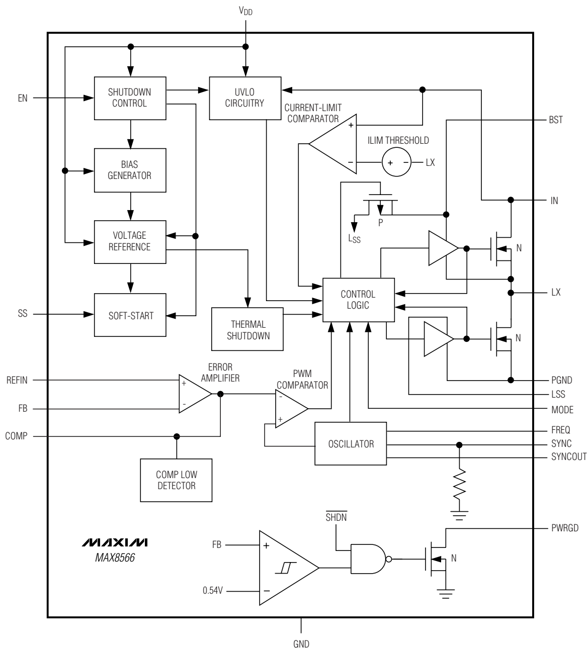
Figure 1. Functional Diagram
