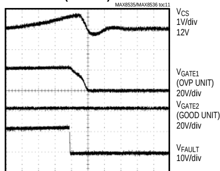
SELECTIVE OVP SHUTDOWN WAVEFORM ( R_1 = 10\Omega )
