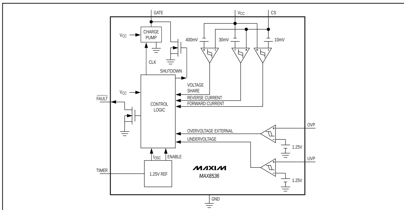
Figure 2. MAX8536 Functional Diagram
