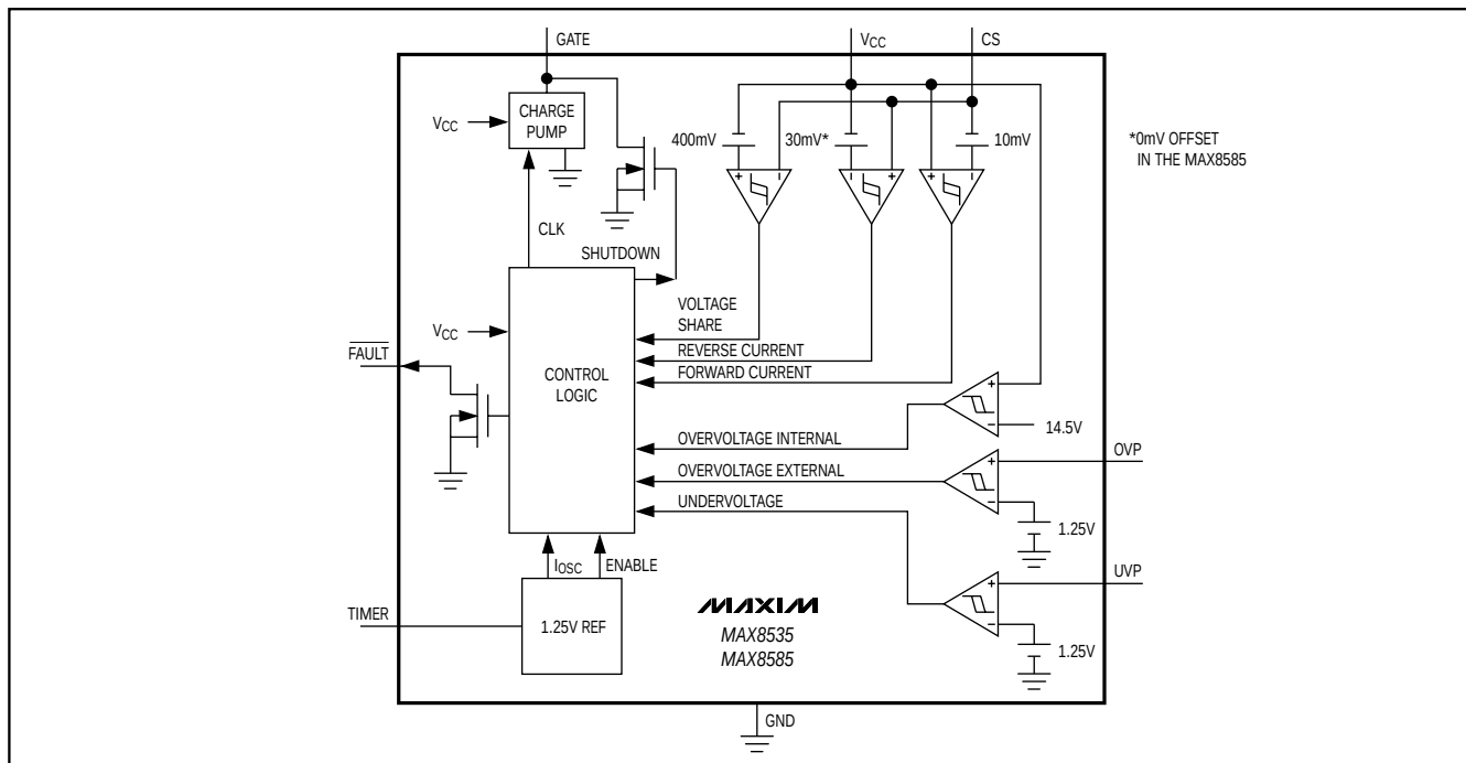
Figure 1. MAX8535/MAX8585 Functional Diagram
