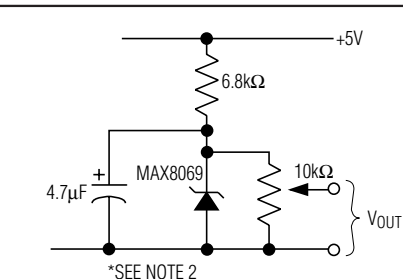
(a) Simple Reference (1.2V or Less)
