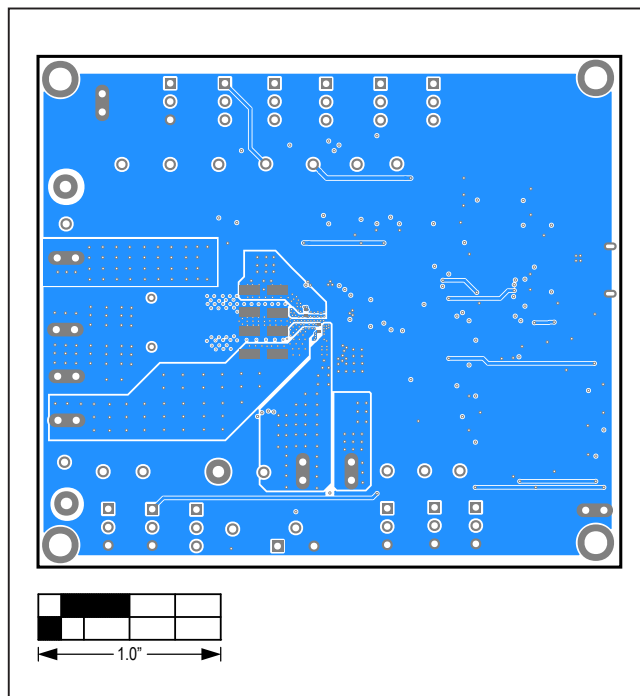
MAX77960/MAX77961 EV Kit PCB Layout – Bottom Layer
