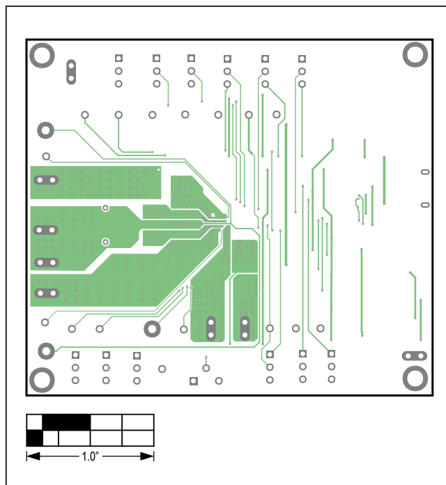
MAX77960/MAX77961 EV Kit PCB Layout – Inner Layer 3
