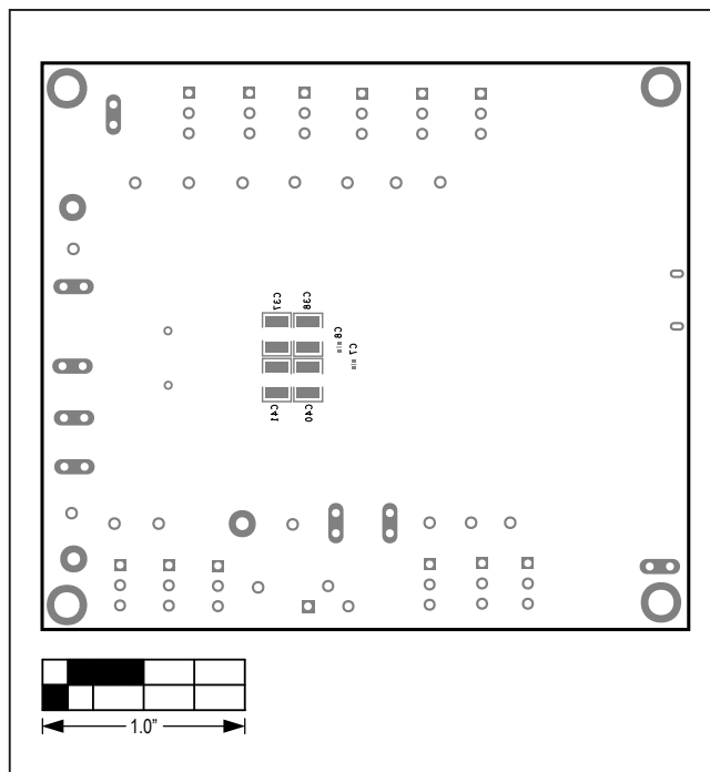
MAX77960/MAX77961 EV Kit PCB Layout – Silkscreen Bottom
