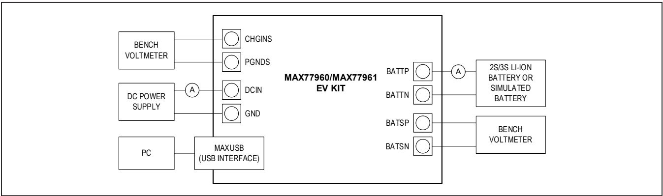
Figure 2. EV Kit Simple Block Diagram
