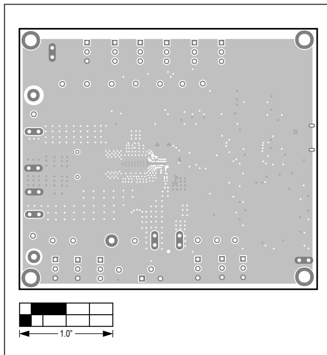
MAX77960/MAX77961 EV Kit PCB Layout – Inner Layer 2
