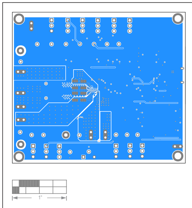
MAX77960B/MAX77961B EV Kit PCB Layout—Bottom Layer
