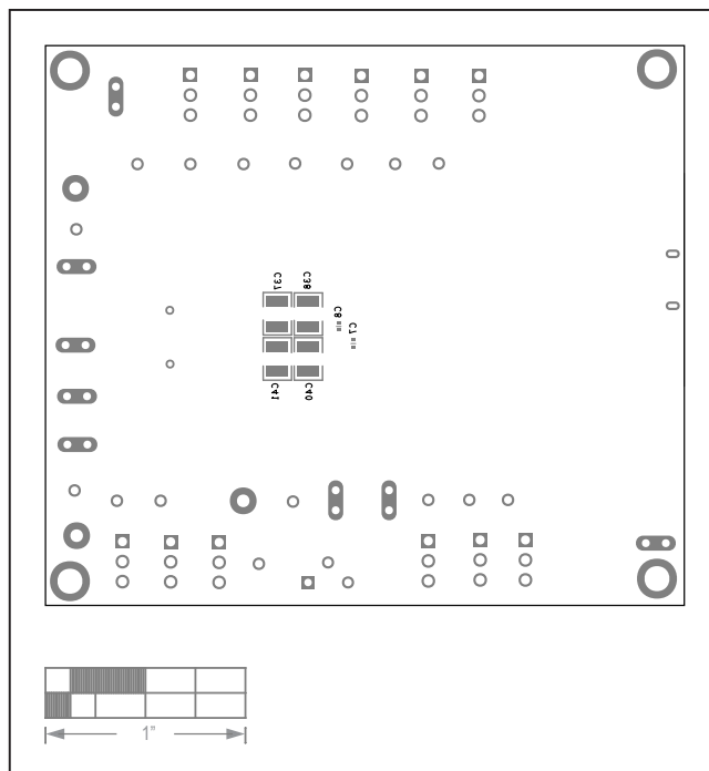
MAX77960B/MAX77961B EV Kit PCB Layout—Silkscreen Bottom
