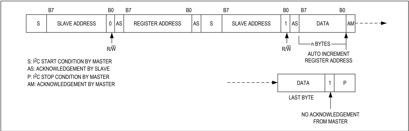
Figure 12. I2C Master Reads After Setting Register Address
