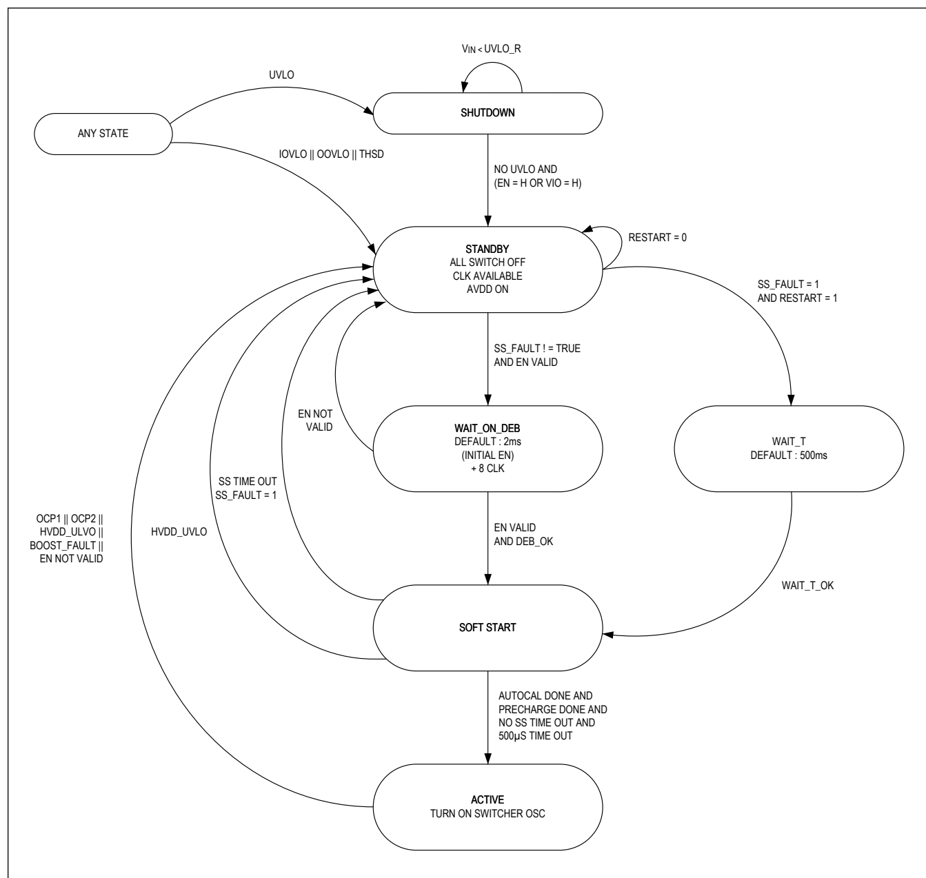
Figure 6. Device State Diagram
