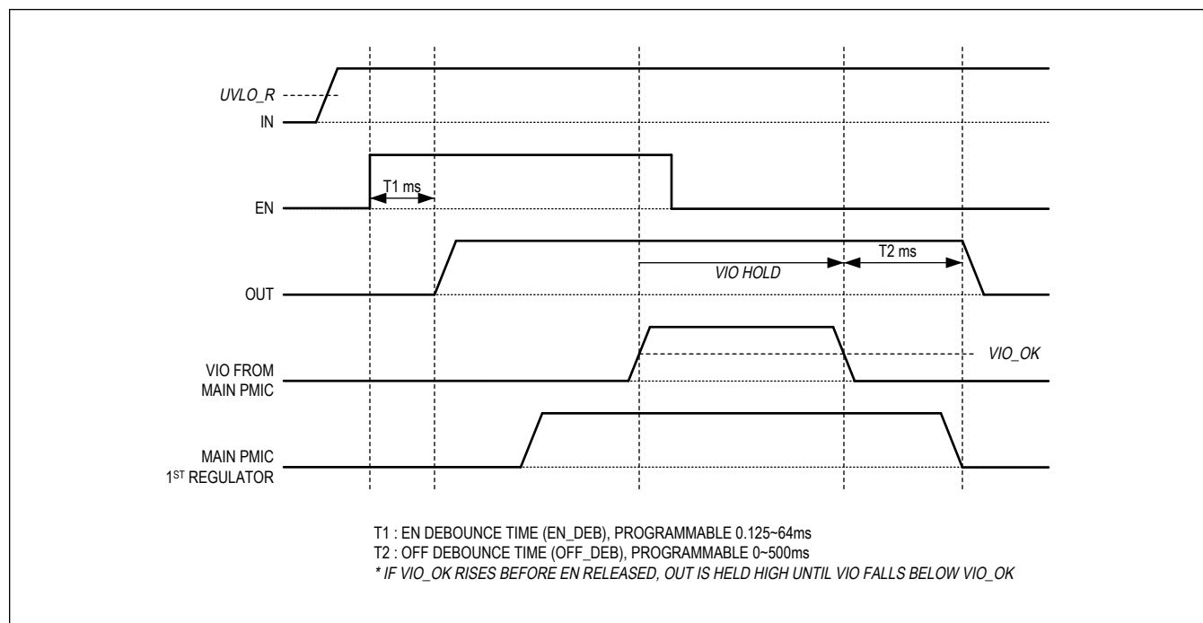
Figure 2. Enable Timing Waveform with VIO Hold
