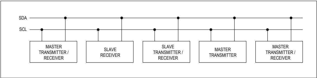
Figure 9. System Configurations
