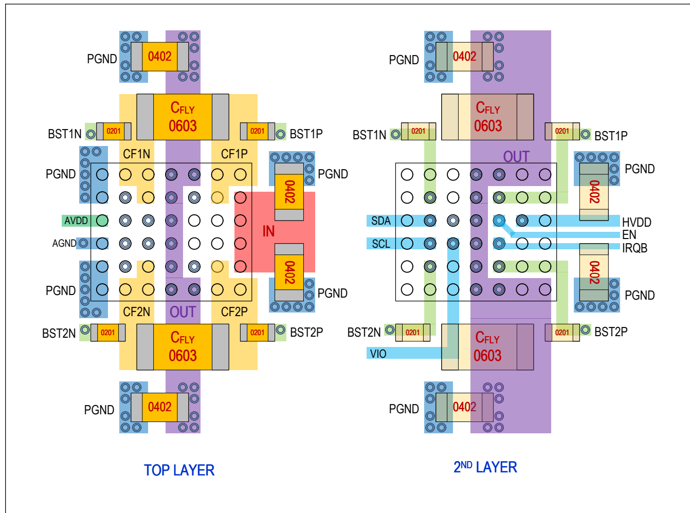
Figure 14. Layout Guide
