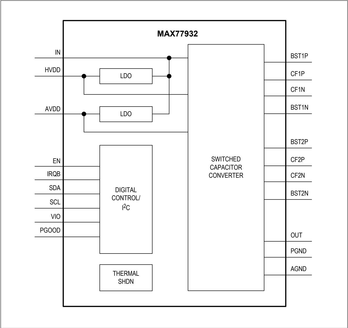
Block Diagram
