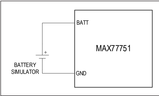
Figure 4. Battery Charger Test with Battery Simulator
