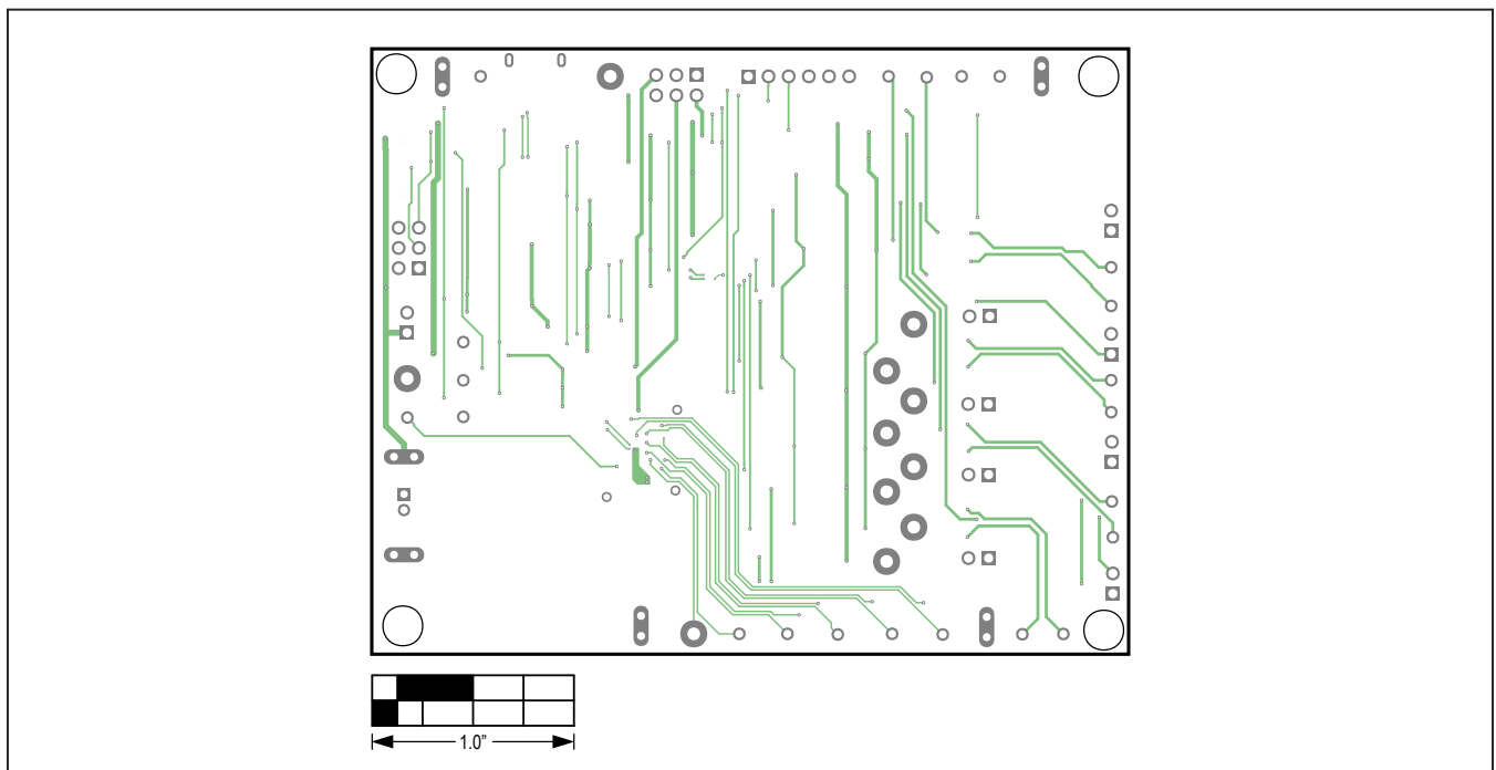
MAX77655 EV Kit PCB Layout – Internal 3
