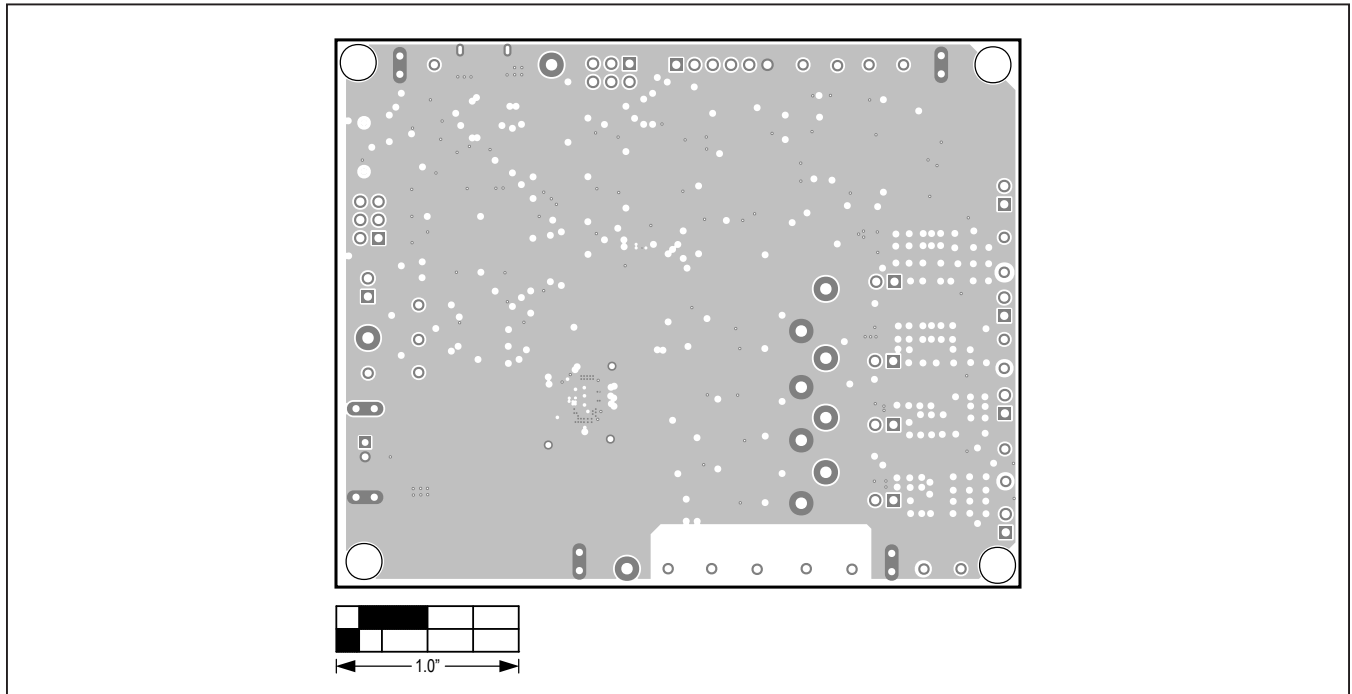
MAX77655 EV Kit PCB Layout – Internal 2
