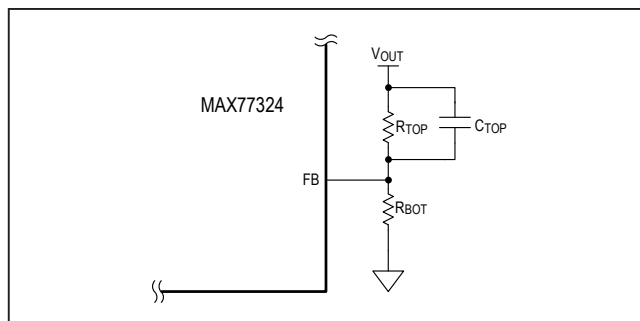
Figure 1. Setting the Output Voltage for MAX77324
