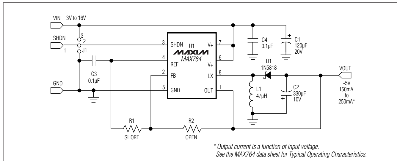
Figure 1. MAX764 EV Kit Schematic
