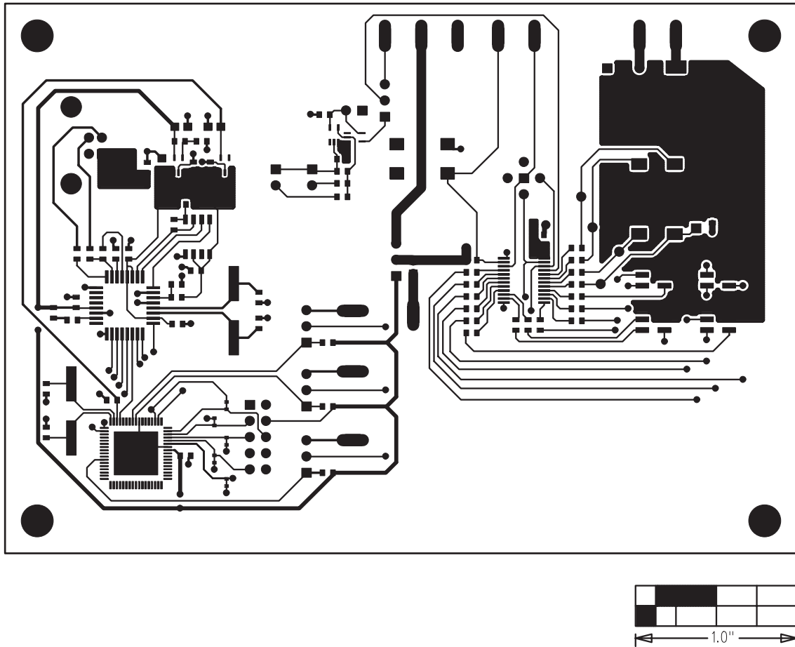
Figure 9. MAX7314 EV Kit PCB Layout—Component Side
