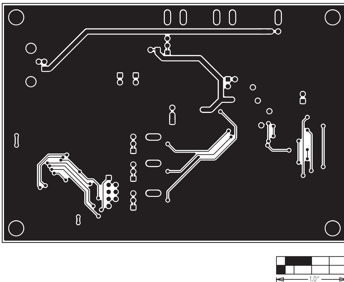
Figure 10. MAX7314 EV Kit PCB Layout—Solder Side
