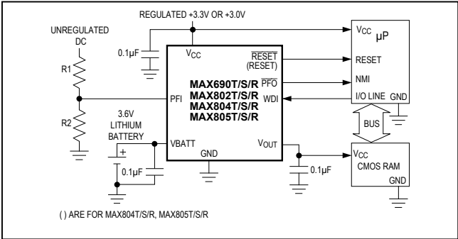
Typical Operating Circuits continued at at end of data sheet.
