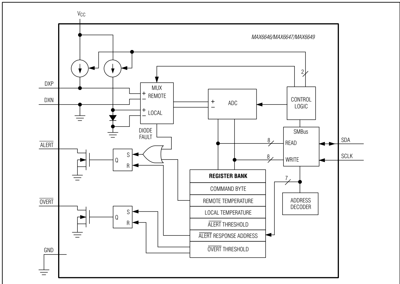
Functional Diagram
