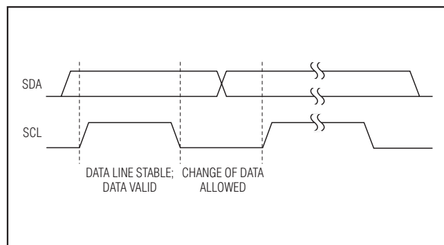
Figure 7. Bit Transfer
