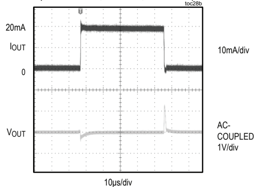
LOAD TRANSIENT ( V_{OUT} = 4.096V , C_{OUT} = 0 , 0 TO 20mA)
