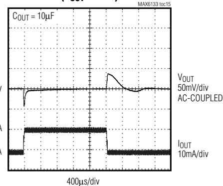
LOAD TRANSIENT ( V_{OUT} = 2.5V )
