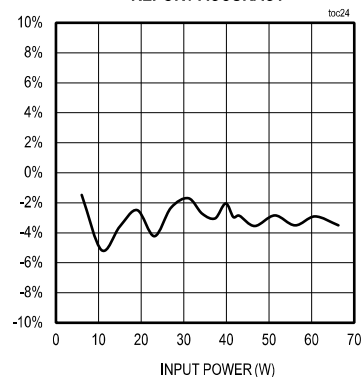
MEC POWER TELEMETRY REPORT ACCURACY
