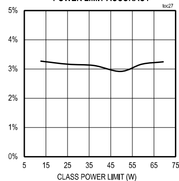
POWER LIMIT ACCURACY
