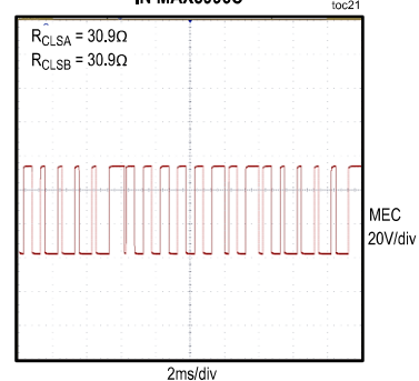
MEC WAVEFORM (CLASS 4, NO LOAD) IN MAX5996C
