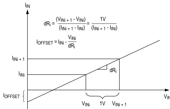
Figure 1. Effective Differential Input Resistance/Offset Current
