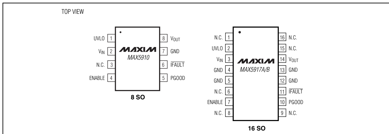
Pin Configurations
