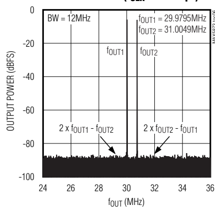
TWO-TONE IMD ( f_{CLK} = 100Mps )
