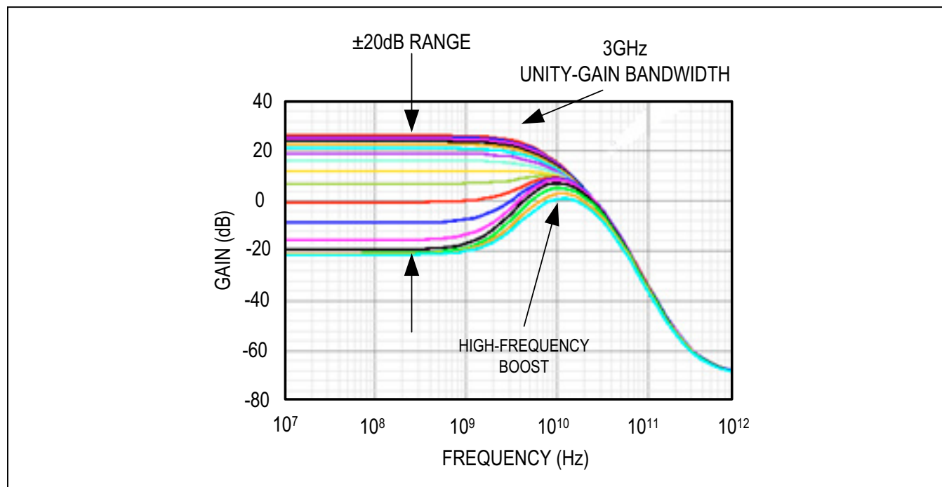
Figure 3. VGA Gain Range
