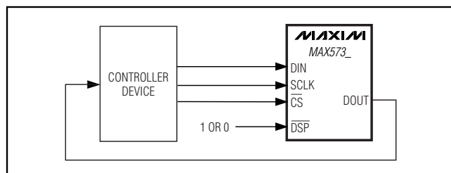
Figure 7. Stand-Alone Configuration
