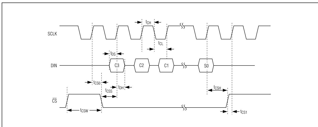
Figure 1. Timing Diagram
