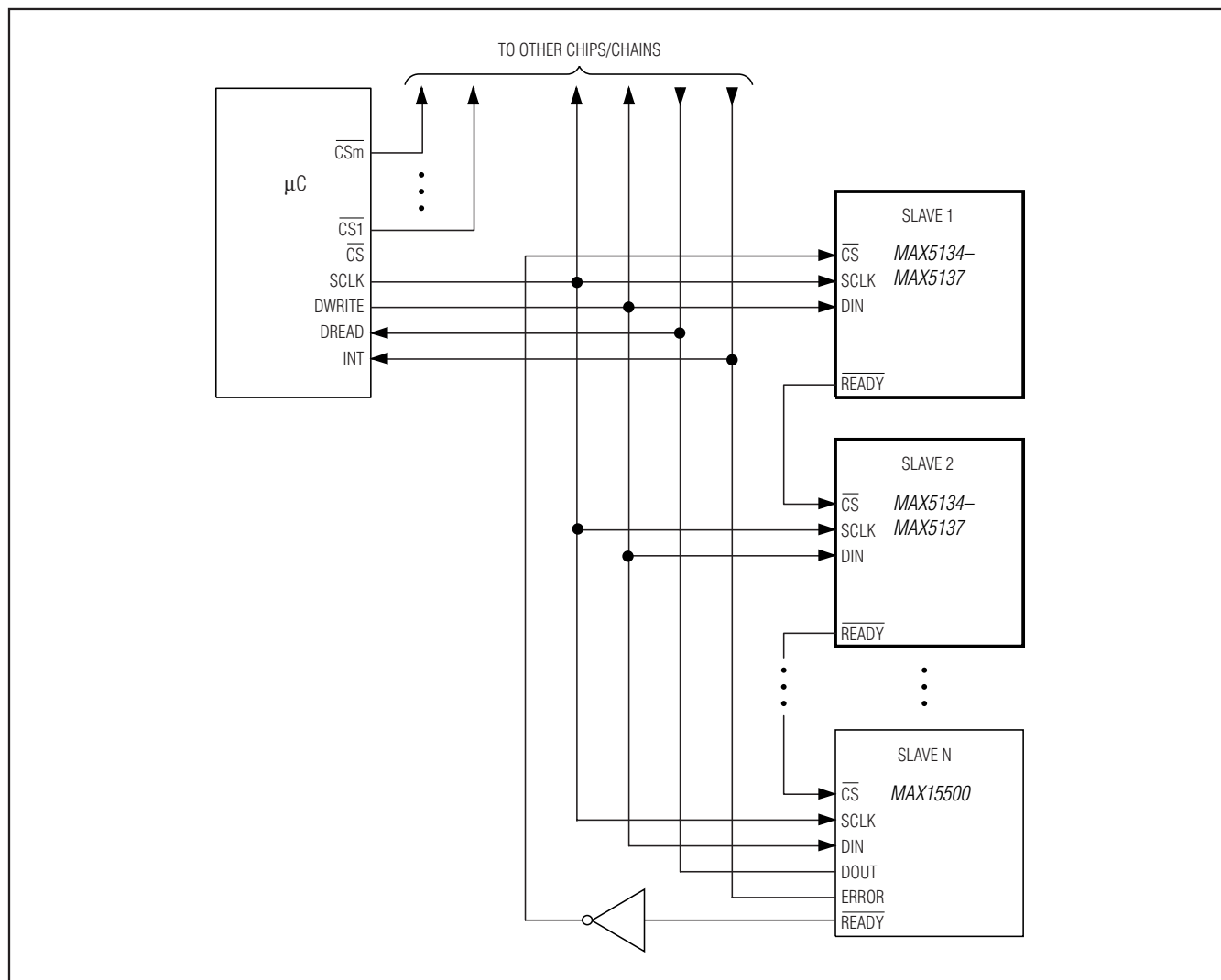
Figure 6. Daisy Chain ( \overline{CS} Not Used)
