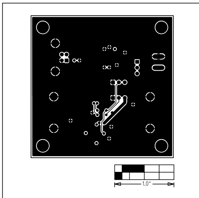
Figure 7. MAX4983E EV Kit PCB Layout—Solder Side
