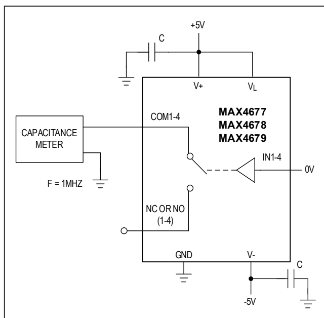
Figure 8b. Channel On-Capacitance
