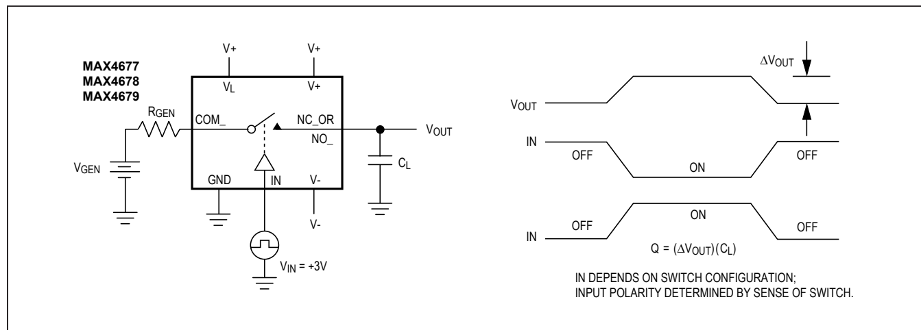
Figure 4. Charge Injection
