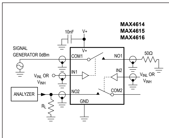
Figure 5. Crosstalk
