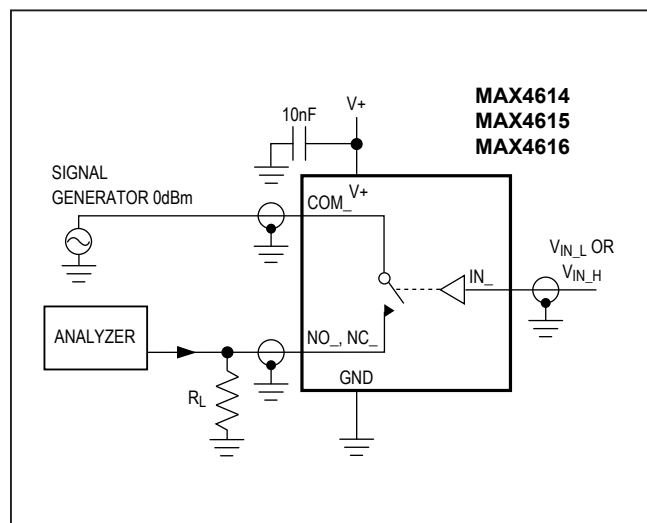
Figure 4. Off-Isolation/On-Channel Bandwidth
