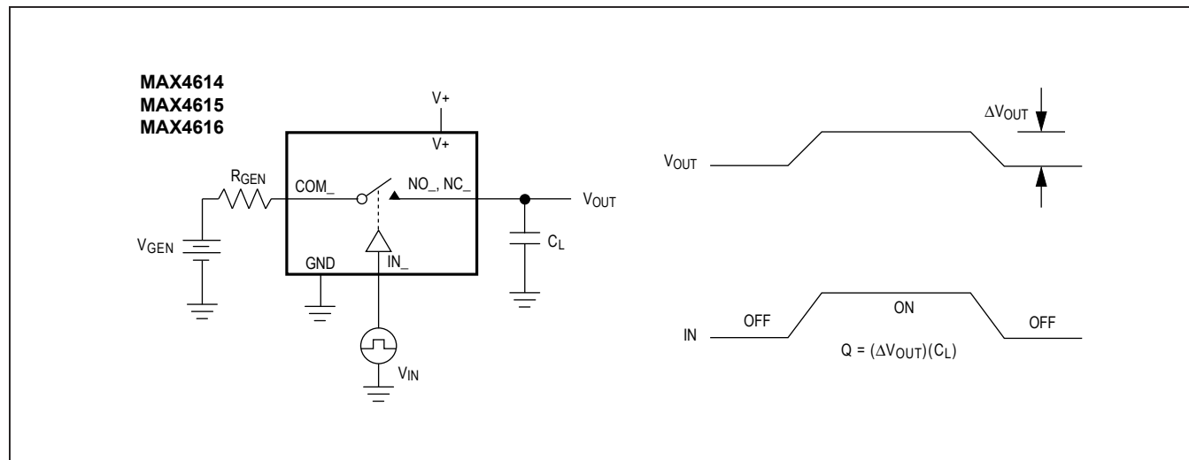
Figure 3. Charge Injection
