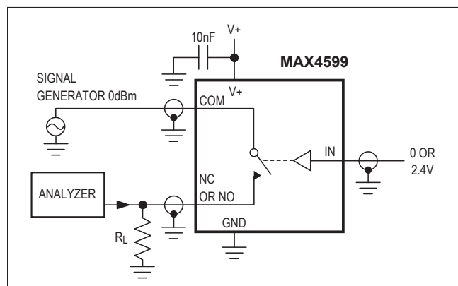
Figure 5. Off-Isolation/On-Channel Bandwidth
