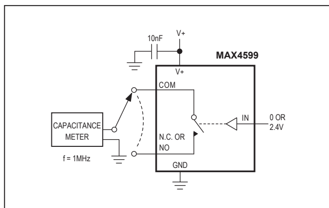
Figure 6. Channel On/Off-Capacitance
