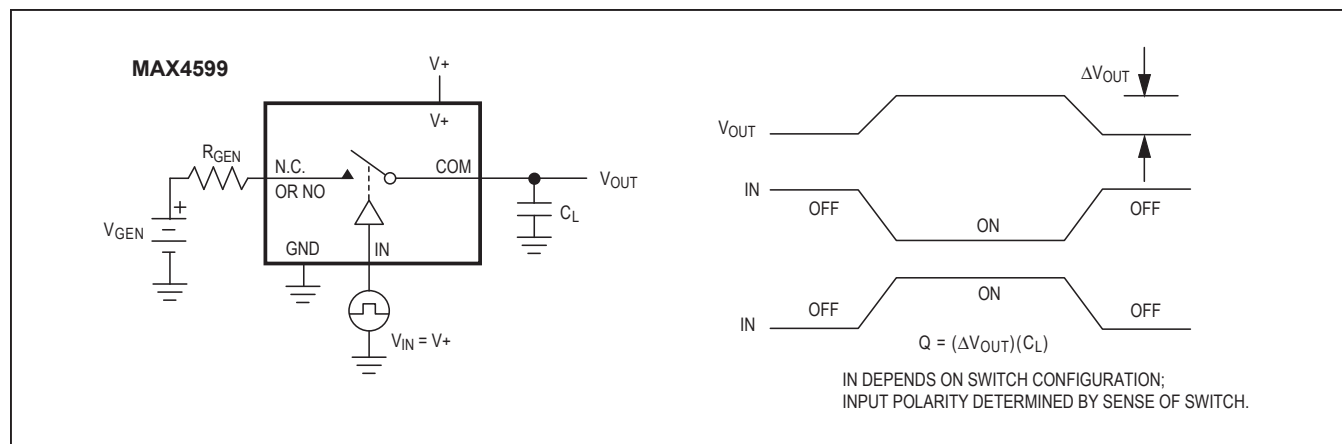
Figure 4. Charge Injection
