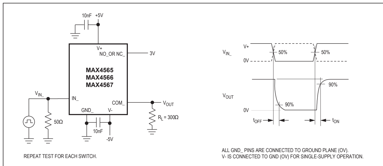
Figure 3. Switching Time
