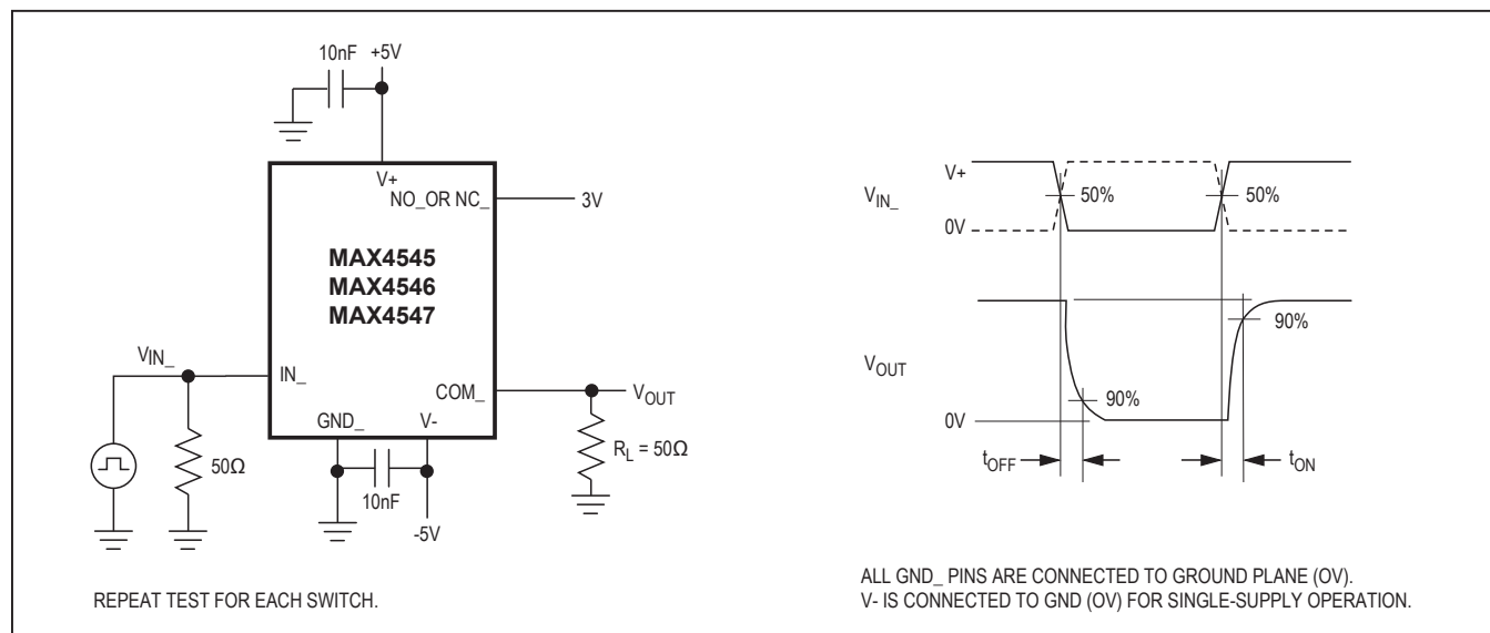
Figure 4. Switching Time
