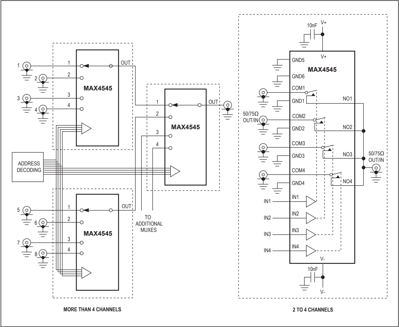
Figure 3. 4-Channel Multiplexer
