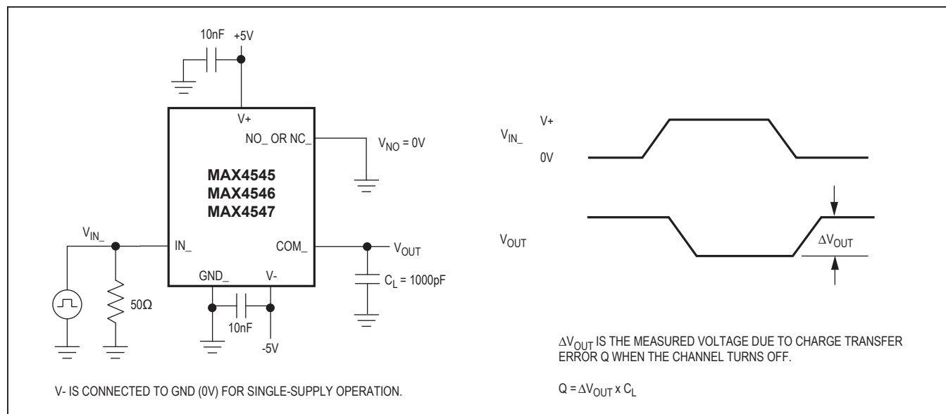
Figure 6. Charge Injection
