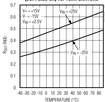
OUTPUT CLAMP RESISTANCE (SUPPLIES ON) vs. TEMPERATURE
