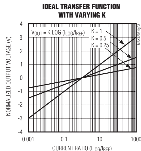
Figure 3. Ideal Transfer Function with Varying K
