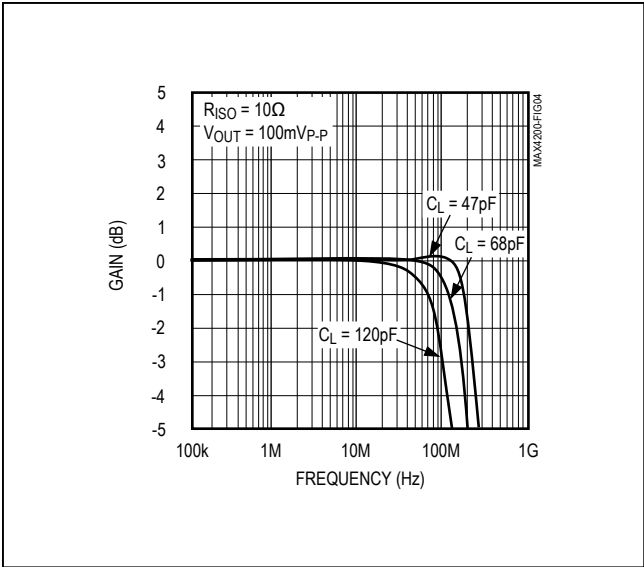
Figure 4. MAX4200/MAX4203 Small-Signal Gain vs. Frequency with Load Capacitance and 10\Omega Isolation Resistor
