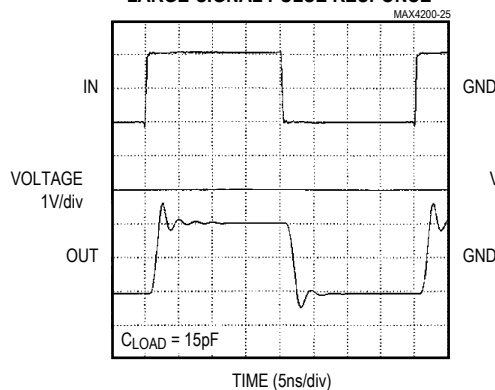
MAX4200/MAX4203 LARGE-SIGNAL PULSE RESPONSE
