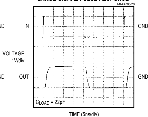
MAX4201/MAX4202/MAX4204/MAX4205 LARGE-SIGNAL PULSE RESPONSE
