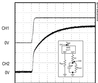
STARTUP DELAY (V BIAS = 5V, I REF = 250nA)
