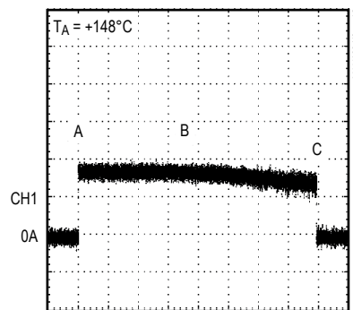
SHORT-CIRCUIT RESPONSE (V BIAS = 5V)
