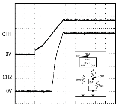
STARTUP DELAY (V BIAS = 2.7V, I REF = 2.5mA)
