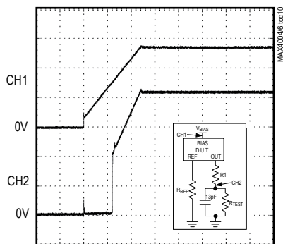
STARTUP DELAY (V BIAS = 2.7V, I REF = 250nA)
