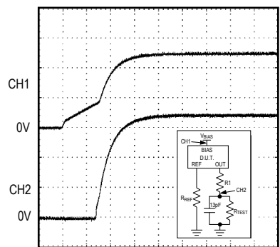
STARTUP DELAY (V BIAS = 5V, I REF = 2.5mA)
