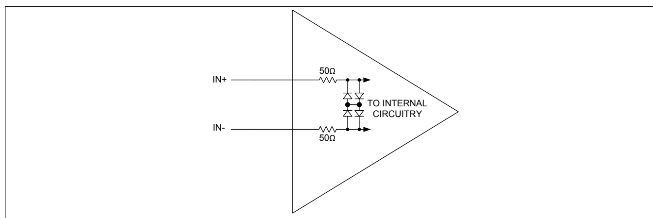
Figure 6. Input Stage Circuitry
